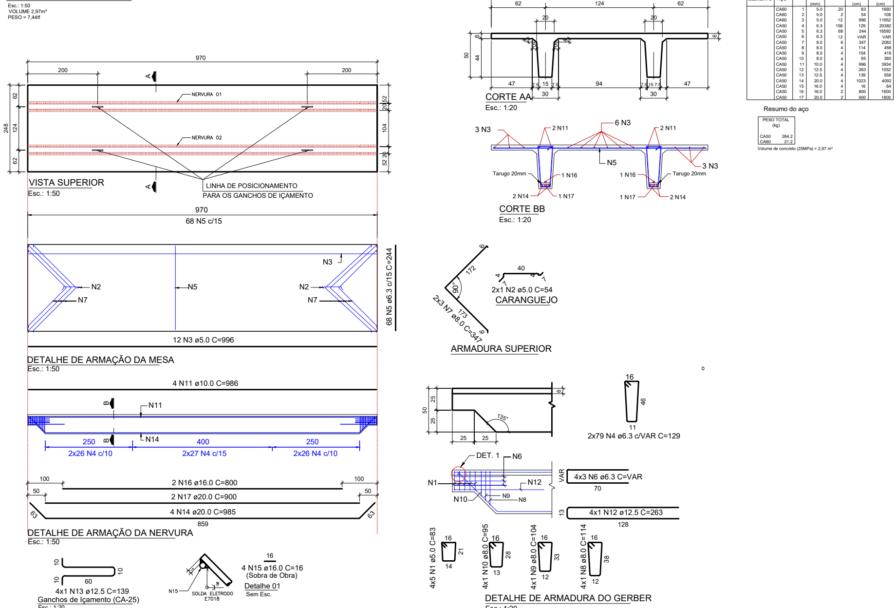
LP-1 (248x30x1000) (x5)
